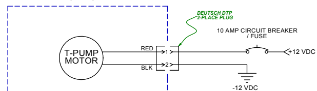
T-SERIES DISCHARGE PUMP ON HOLDING TANK
