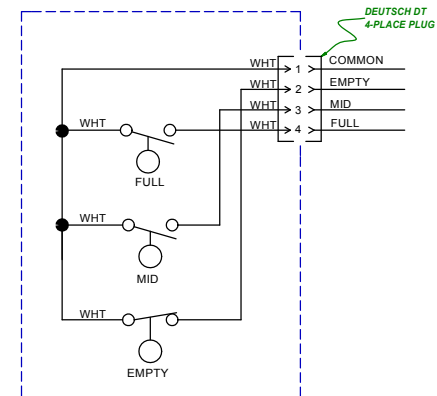
BLACK WATER HOLDING TANK FLOAT SWITCH ARRAY
