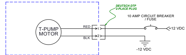
T-SERIES DISCHARGE PUMP ON HOLDING TANK
