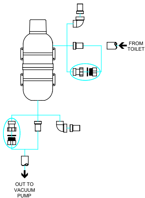
TYPICAL VERTICAL WALL MOUNT
