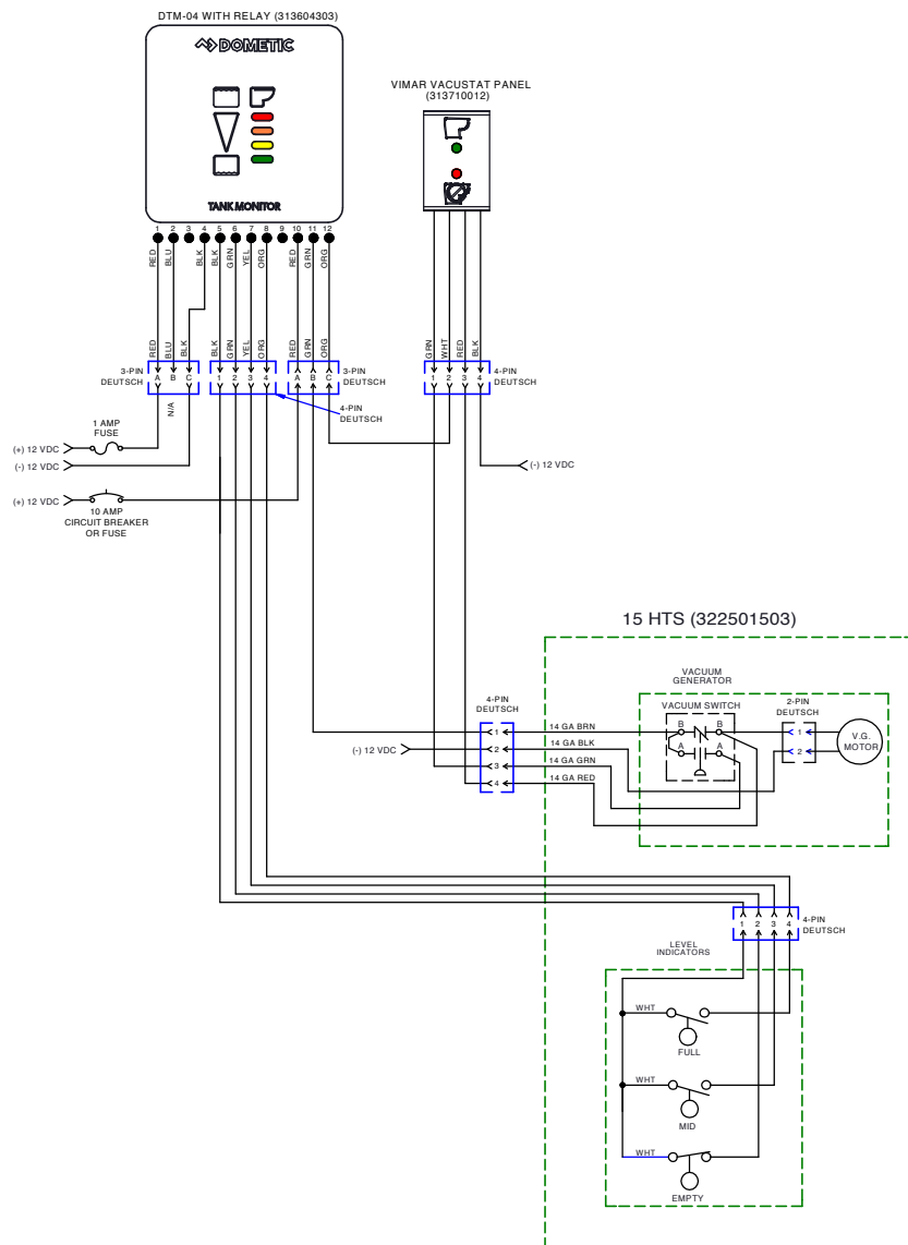
CHAPARRAL 327 WITHOUT OVERBOARD DISCHARGE
