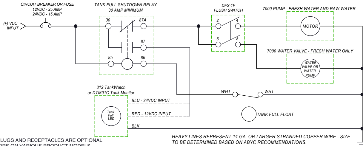
7000 SERIES FRESH/RAW WATER WIRING DIAGRAM - WITH TANK FULL RELAY
