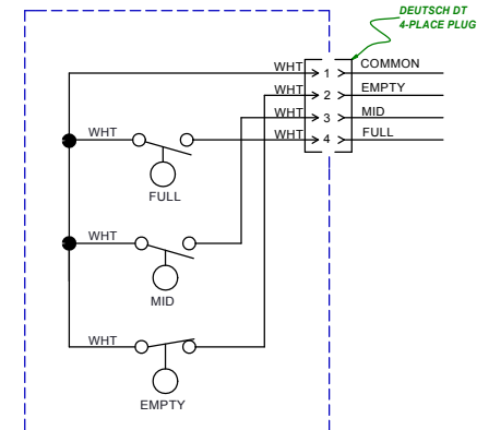
BLACK WATER HOLDING TANK FLOAT SWITCH ARRAY
